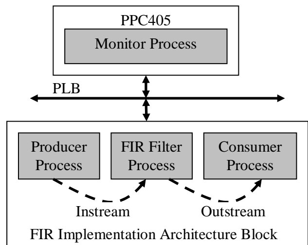
Figure 2: FIR Hardware Implementation.
